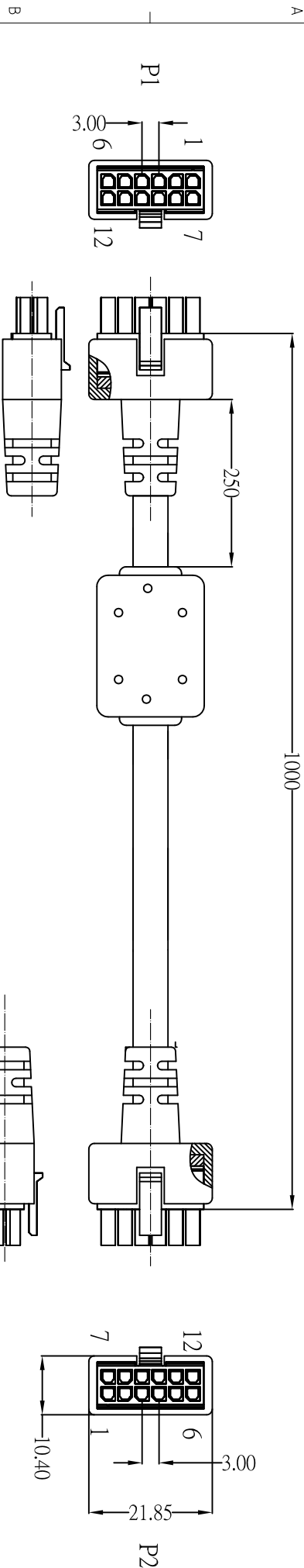
HOUSING C3030HF-2x6P
