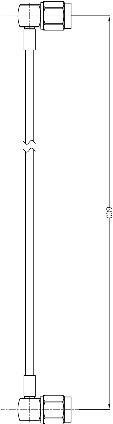
SMA RIGHT-ANGLE PLUG
