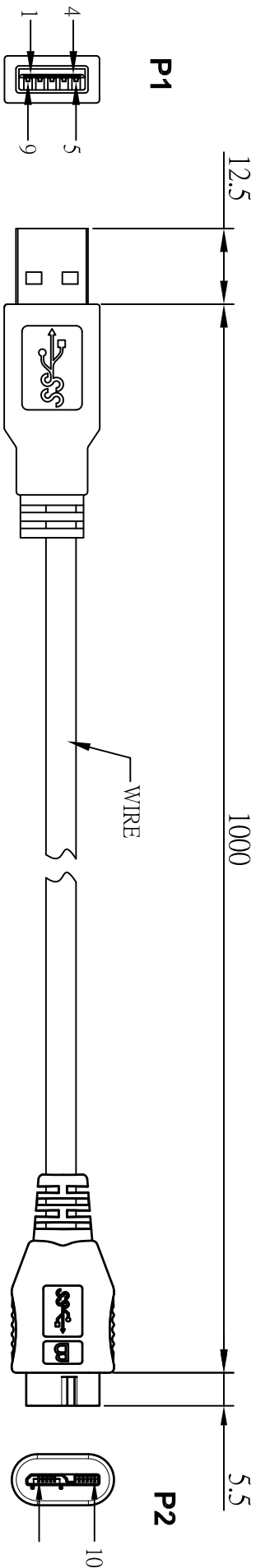
USB3.0 MICRO-B PLUG
