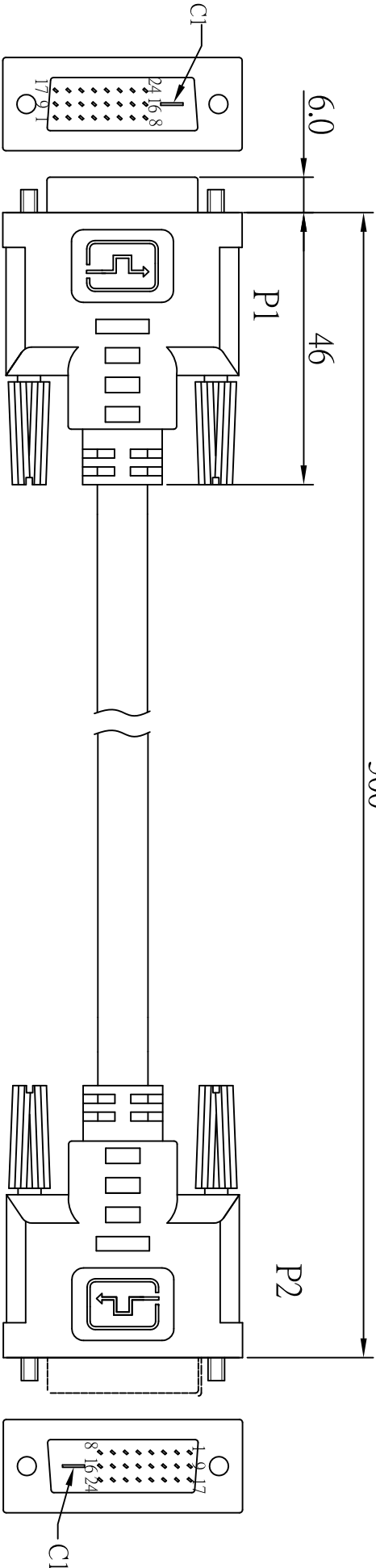
DVI 24PIN+1C PLUG FULL SHIELD
