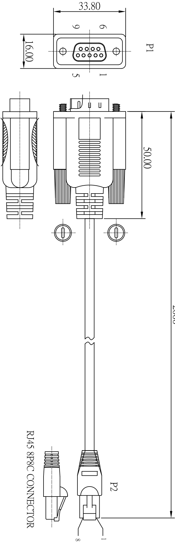
DB 9PIN PLUG
